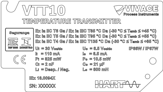
Figura 5.2 – Plaqueta Ex ia do VTT10-FH.
