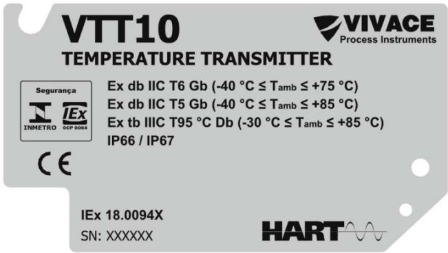
Figura 5.1 – Plaqueta Ex d do VTT10-FH.
